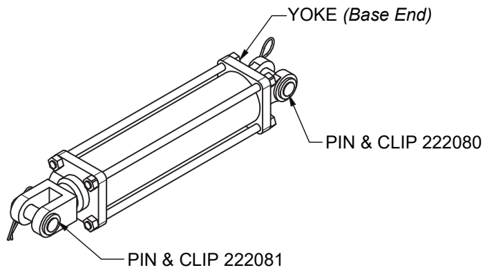
222071 Cylinder, Hydraulic, 3.50 X 1.25 X 12
